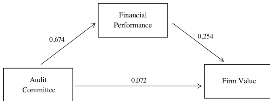
Figure 1 Path analysis
